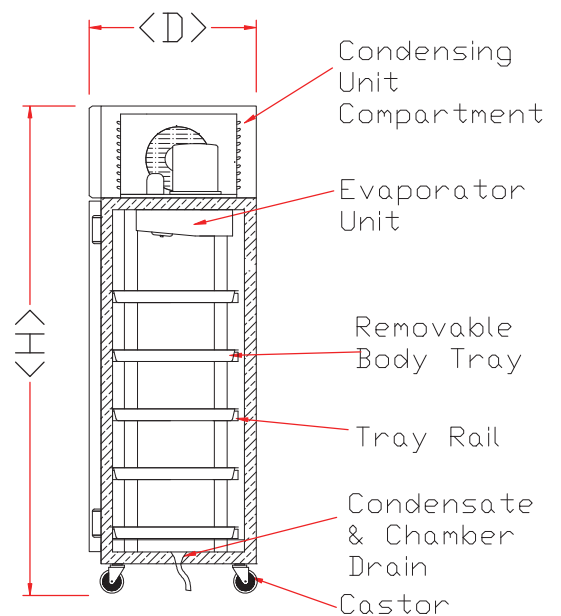
Side Cross Section View
